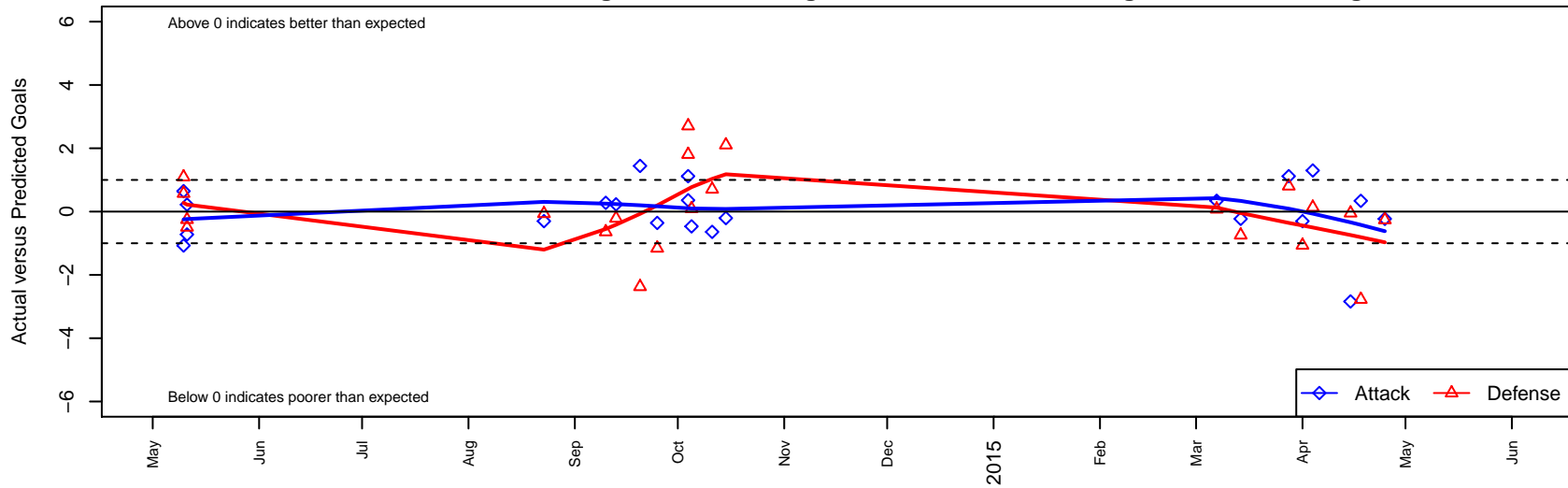
Boise Nationals SC Blue G01 Dots are actual minus expected GF (blue circles) and GA (red triangles). Blue line is smoothed change in attack strength. Red is smoothed change in defense strength.
